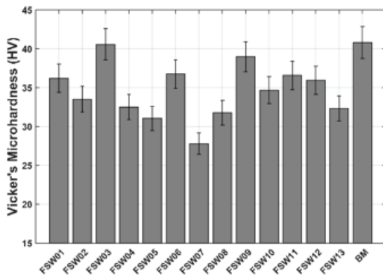
Figure 1. Microhardness of the base material and friction stir welded specimens.
