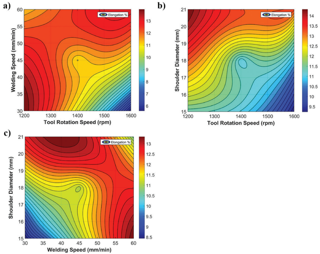
Figure 14. Effect of friction stir welding process parameters on % elongation (a) tool rotation speed and welding speed; (b) tool rotation speed and shoulder diameter; (c) welding speed and shoulder diameter.
