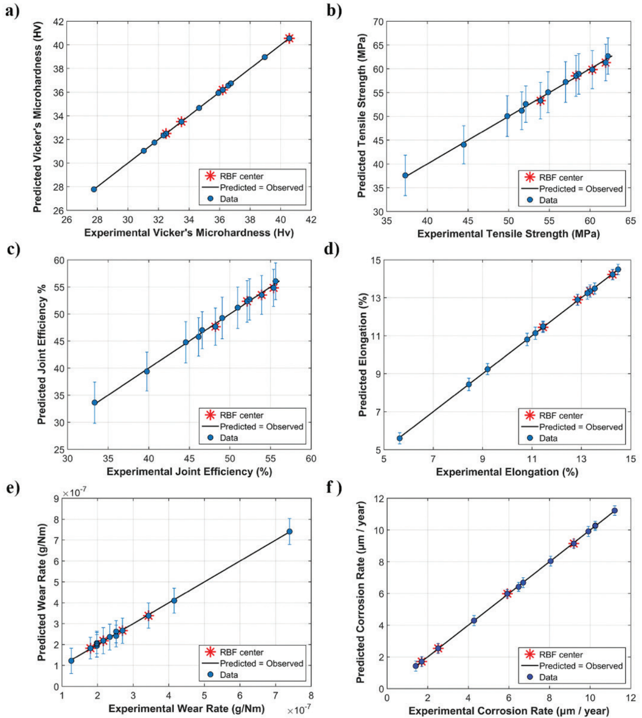
Figure 10. Plot of experimental vs predicted values of (a) microhardness; (b) tensile strength; (c) joint efficiency; (d) % elongation; (e) wear rate; (f) corrosion rate.
