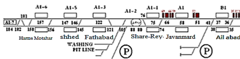
Figure 3. Schematic layout of stations, railway blocks, and terminals in a case study (source: Tehran metro comprehensive system)
