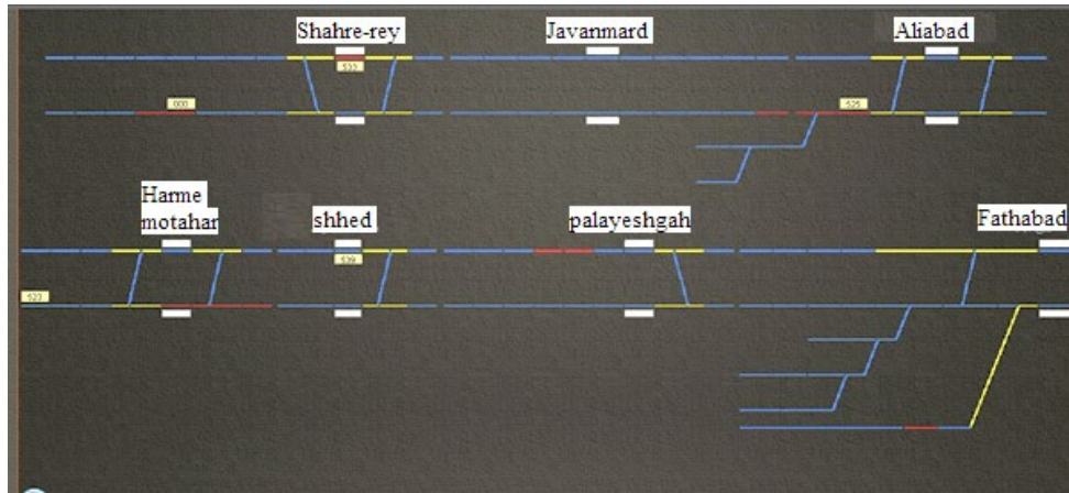
Figure 5: schematic view of the southern section of line 1 of the Tehran metro, which is based on the output of the comprehensive system of the timetable
