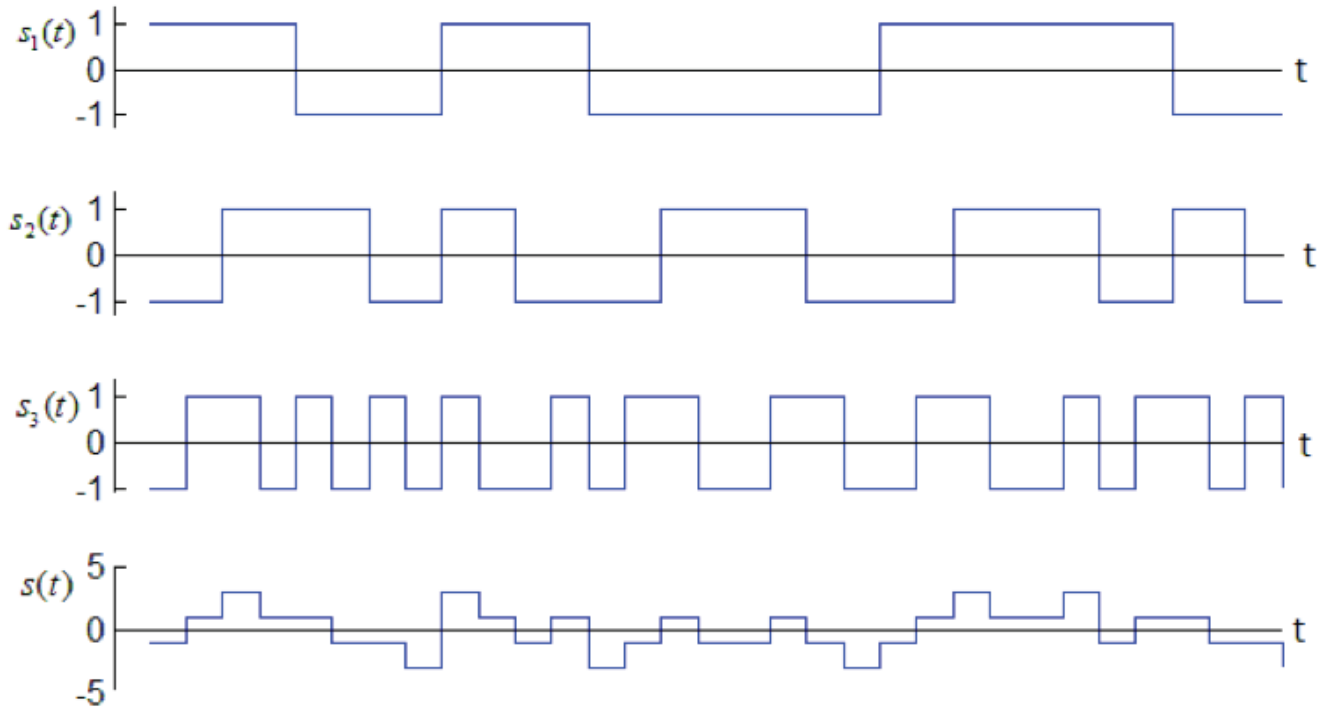
Figure 6. Subchannel signals s_1(t) , s_2(t) , s_3(t) and theirs sum s(t) .
